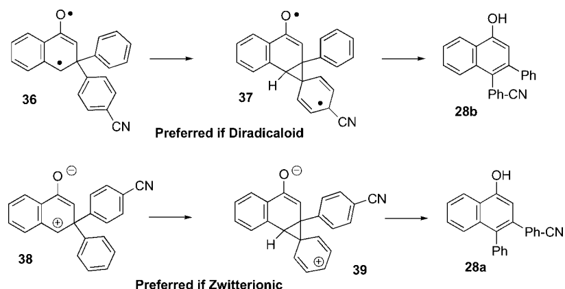
Scheme 5. Phenyl migration preference signifies zwitterionic character; dependence of migrations on zwitterionic vs. diradical character.
