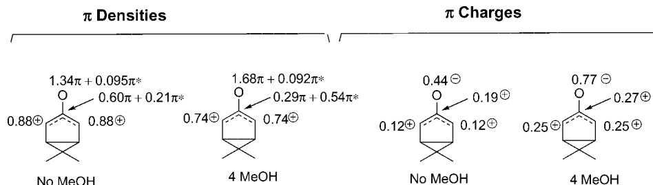
Figure 3. Electron densities and charges in the \pi -system.
