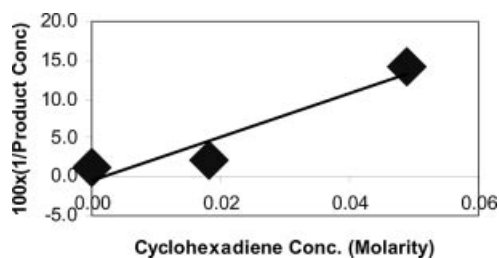
Figure 1. Inverse of conversion vs. quencher concentration.
