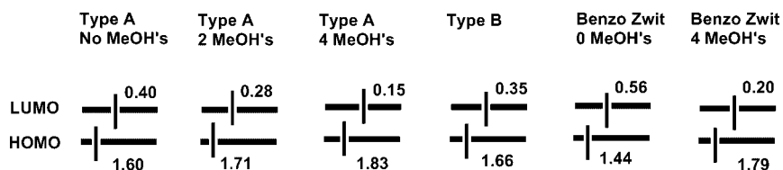
Figure 2. Natural orbital occupancies.
