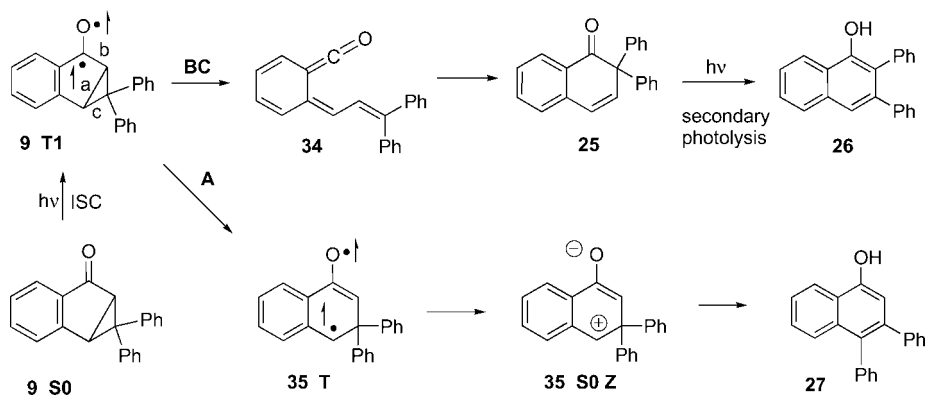
Scheme 4. Postulated mechanisms in the photolysis of benzobicyclic ketone 9 .
